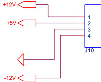
Additional Power Output, Phoenix Contact type FFKDS
