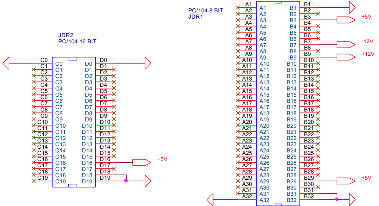
PC/104 standard connectors, Power Output Pin-out
