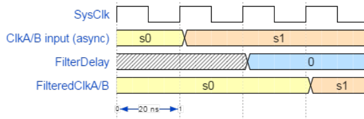
Figure 8: ClkA, ClkB or IX input sampling with filter disabled ( F = 0 )
